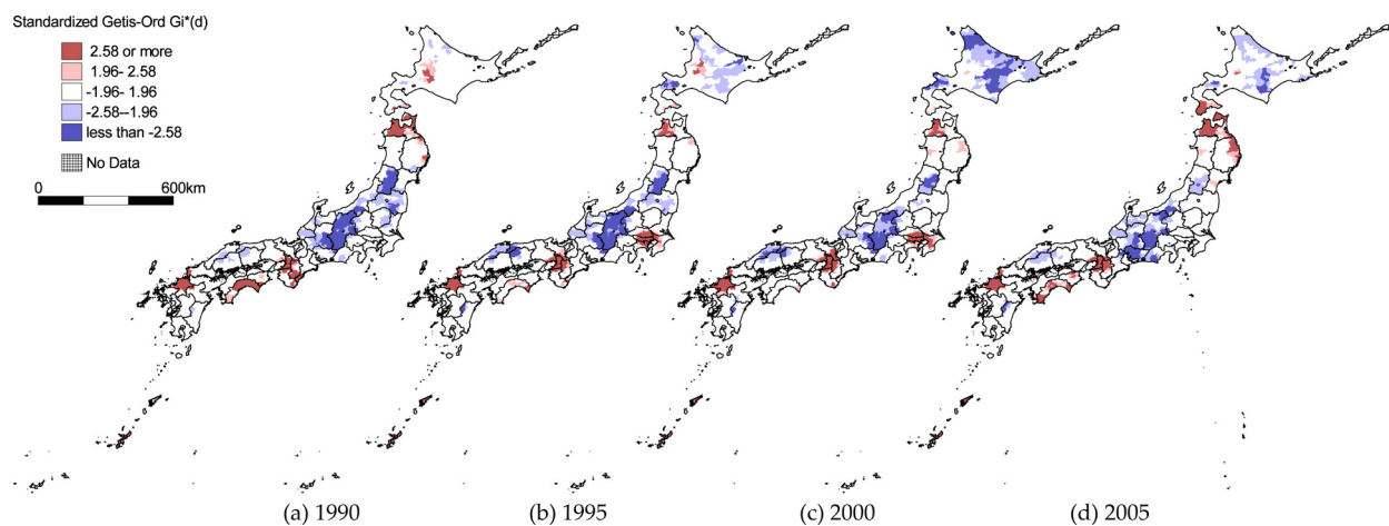
Figure 4: Standardized Getis–Ord G_i^*(d) ( d = 30 km)
